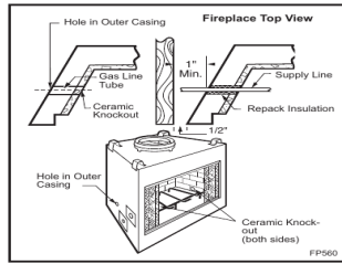
Fig. 27 Gas line access.
